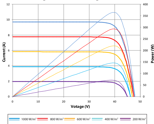
Current-Voltage & Power-Voltage Curve (365S)
