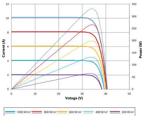
Current-Voltage & Power-Voltage Curve (330S)
