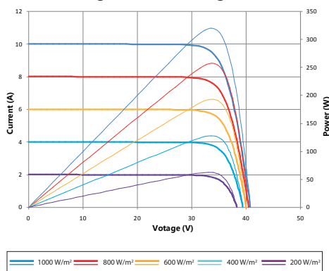
Current-Voltage & Power-Voltage Curve (320S)
