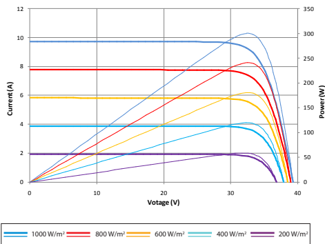
Current-Voltage & Power-Voltage Curve (300S)
